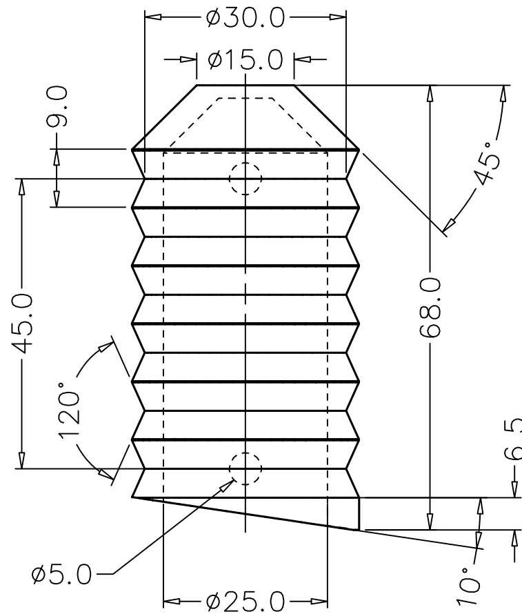
STANDARD INSERT-GRAY P/NO: CCP-03
